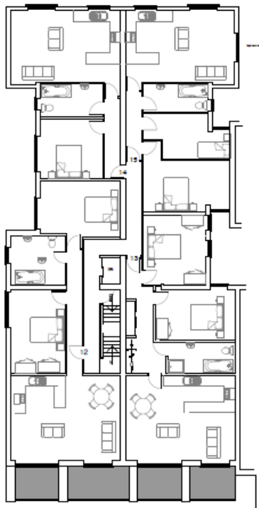
Third Floor Plan 1:100
